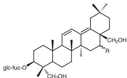
saikosaponin b 1 : R = β-OH saikosaponin b 2 : R = α-OH (サイコ)
