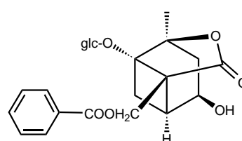
albiflorin (シャクヤク)
