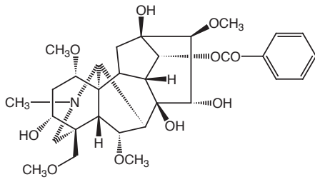
benzoylmesaconine (ブシ末)
