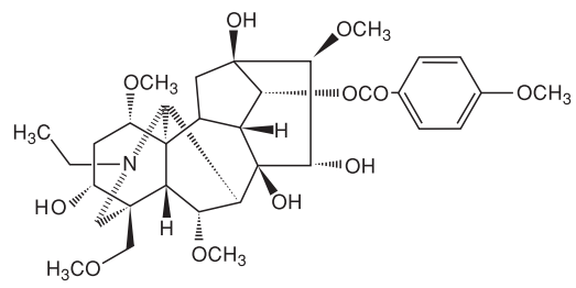
14-anisoylaconine (ブシ末)
