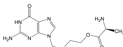
類縁物質 H (Acyclovir alaninate)
