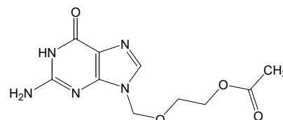
類縁物質 I (Acyclovir related compound A)
