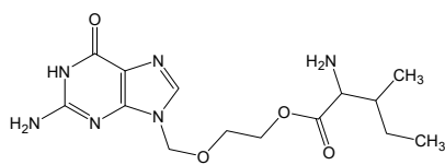
類縁物質 J (Acyclovir isoleucinate)
