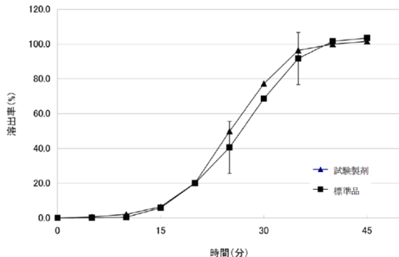
pH6.8 (75rpm)
