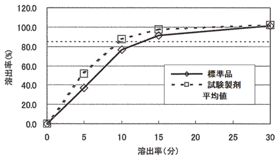
pH6.8 (100rpm)
