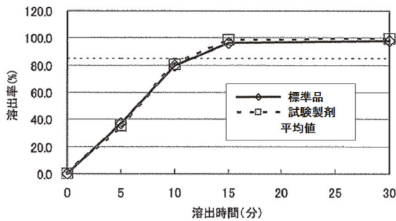
pH1.2 (50rpm)
